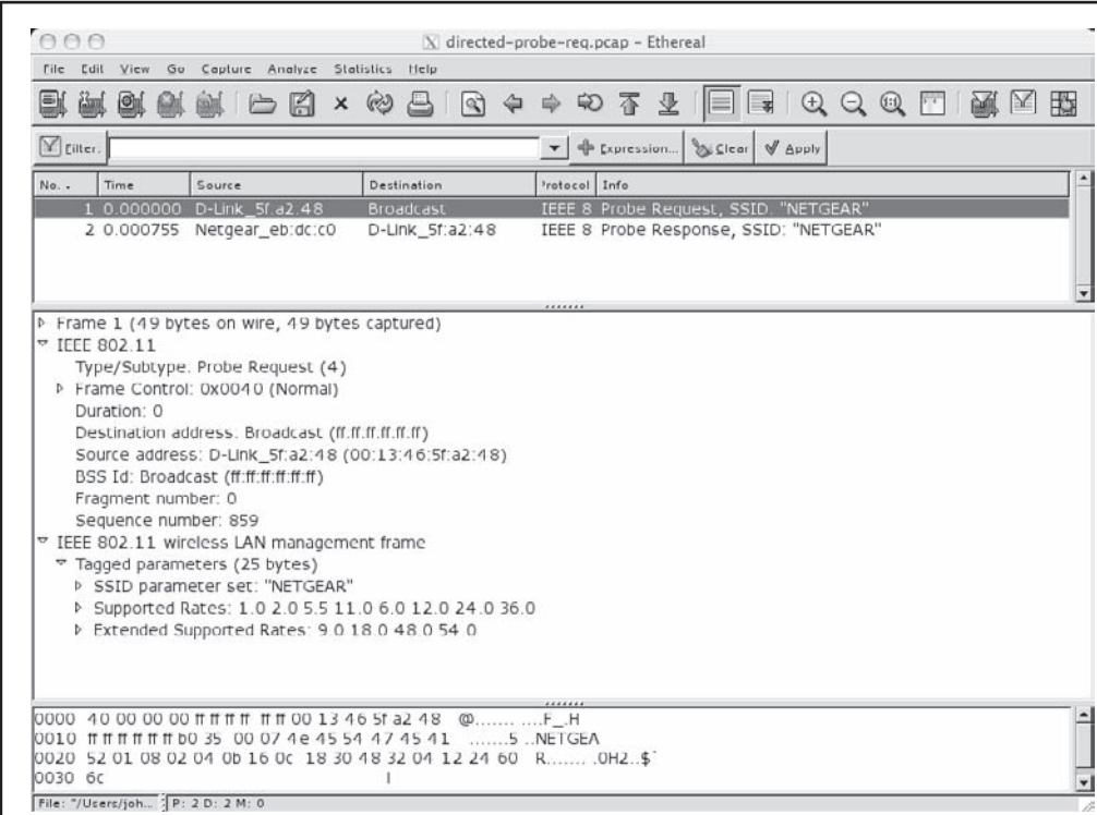
Figure 1-3 A directed probe request—note the addition of an SSID parameter.
