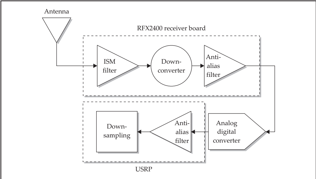
Figure 9-1 USRP2 FPGA processing receive path
